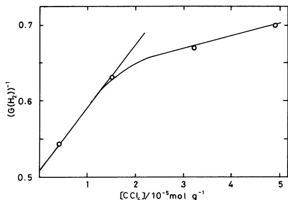
Fig. 8. 1/G(H_2) vs. [CCl_4] . Calculated from the data shown in Fig. 3.
